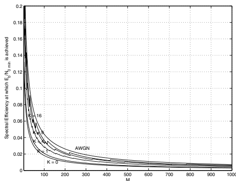
Fig. 5. Spectral efficiency at which E_b/N_{0\min} is achieved vs. M for M -ary FSK in the AWGN channel and noncoherent Rician fading channels with Rician factors K = 0, 1, 4, 9, 16 .
