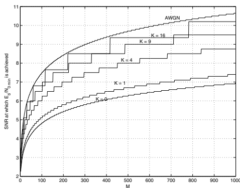
Fig. 6. SNR at which E_b/N_{0\min} is achieved vs. M for M -ary FSK in the AWGN channel and noncoherent Rician fading channels with Rician factors K = 0, 1, 4, 9, 16 .
