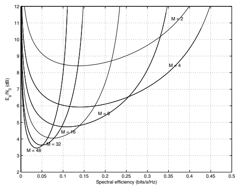
Fig. 2. Bit energy E_b/N_0 vs. Spectral efficiency C(E_b/N_0) for energy-detected M -ary FSK in the coherent Rician fading channel with Rician factor K = 1 .
