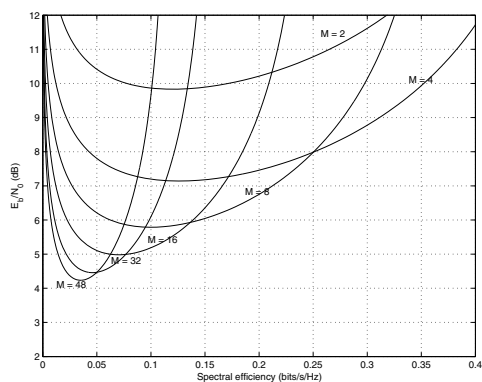
Fig. 3. Bit energy E_b/N_0 vs. Spectral efficiency C(E_b/N_0) for energy-detected M -ary FSK in the noncoherent Rician fading channel with Rician factor K = 1 .
